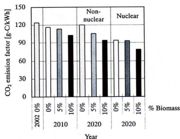
Fig. 10. CO 2 emission factor of power system
