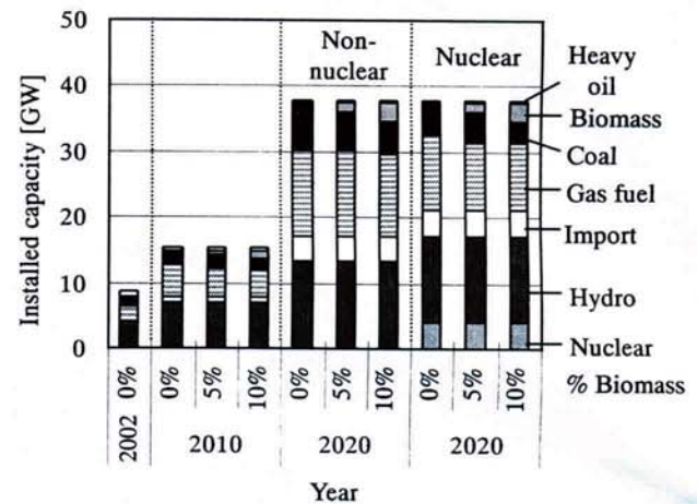
Fig. 6. Optimum installed capacity of power generations
