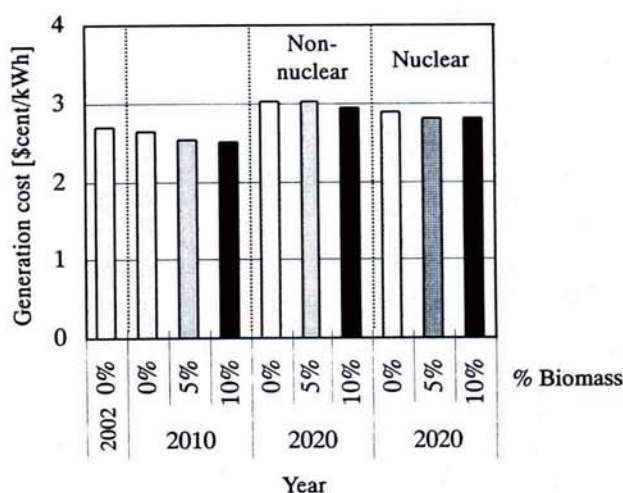
Fig. 9. Generation cost of power system
